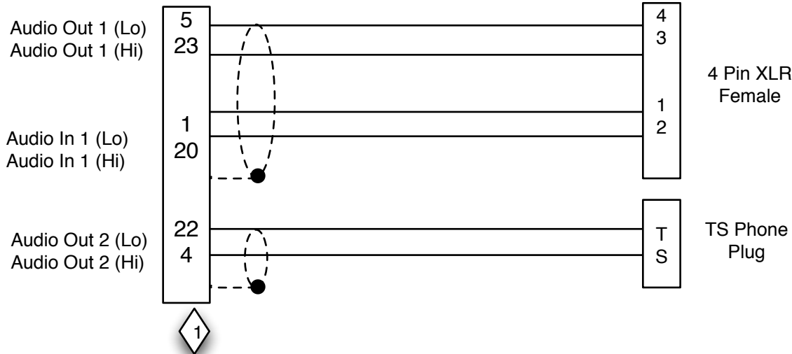
DB37 Connector
